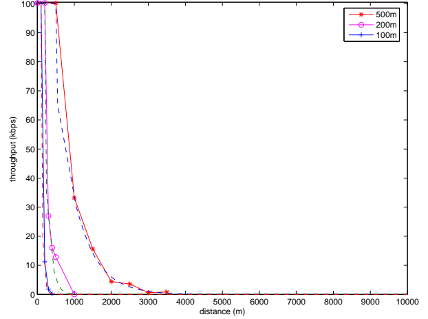
Figure 2. Average throughput of a receiver for different transmission ranges: total density \rho_1 = 5 \times 4 veh/km, \mu = 10\% , inter-packet delay t = 0.02 s, packet size 230 bytes. The corresponding dashed lines are theoretical values obtained from connectivity models.
