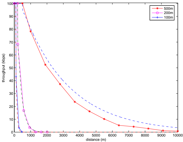
Figure 1. Average throughput of a receiver for different transmission ranges: total density \rho_1 = 14 \times 4 veh/km, \mu = 10\% , inter-packet delay t = 0.02 s, packet size 230 bytes. The corresponding dashed lines are theoretical values obtained from connectivity models.
